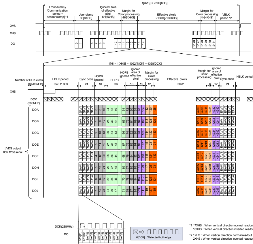
Readout Pixel Image Diagram (4096 × 2160)
