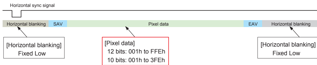
Readout Drive Timing
