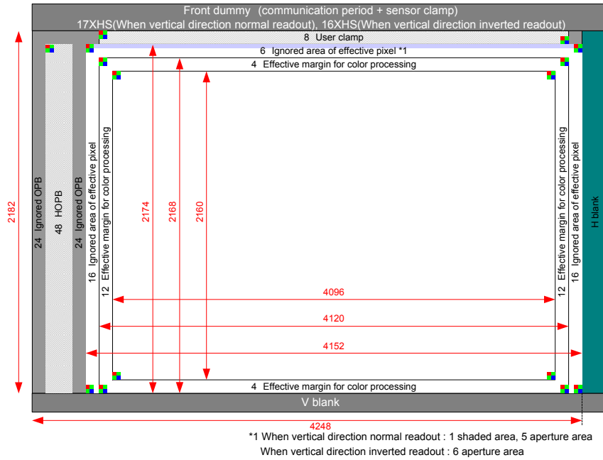
Readout Pixel Image Diagram (4096 × 2160)
