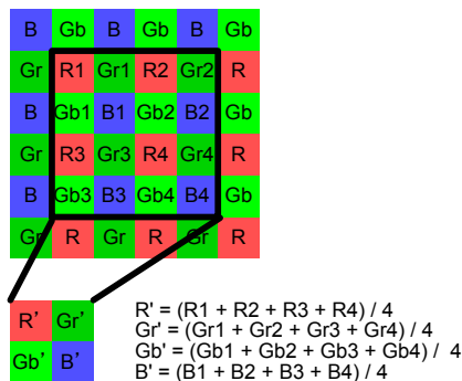
Horizontal/Vertical 2/2-line Binning Image
