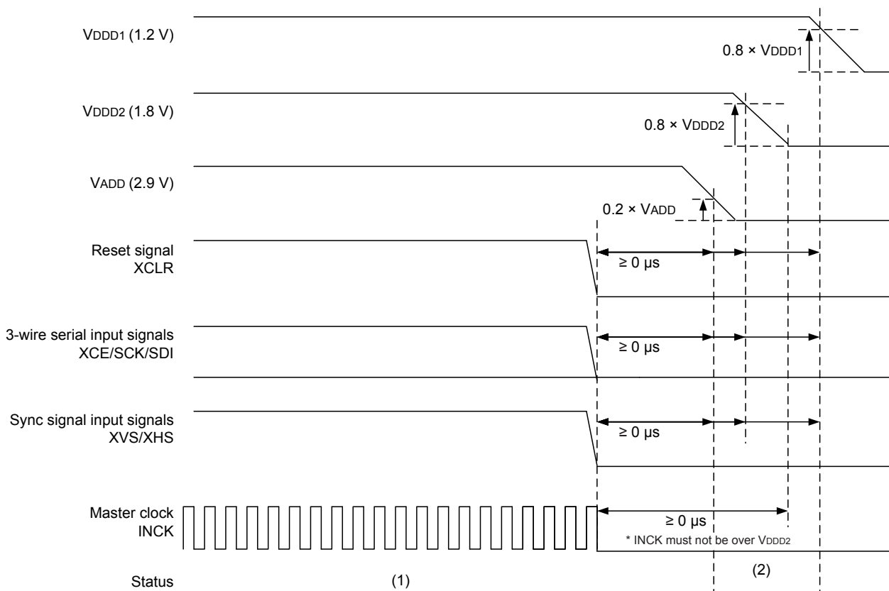
Power-off Sequence
