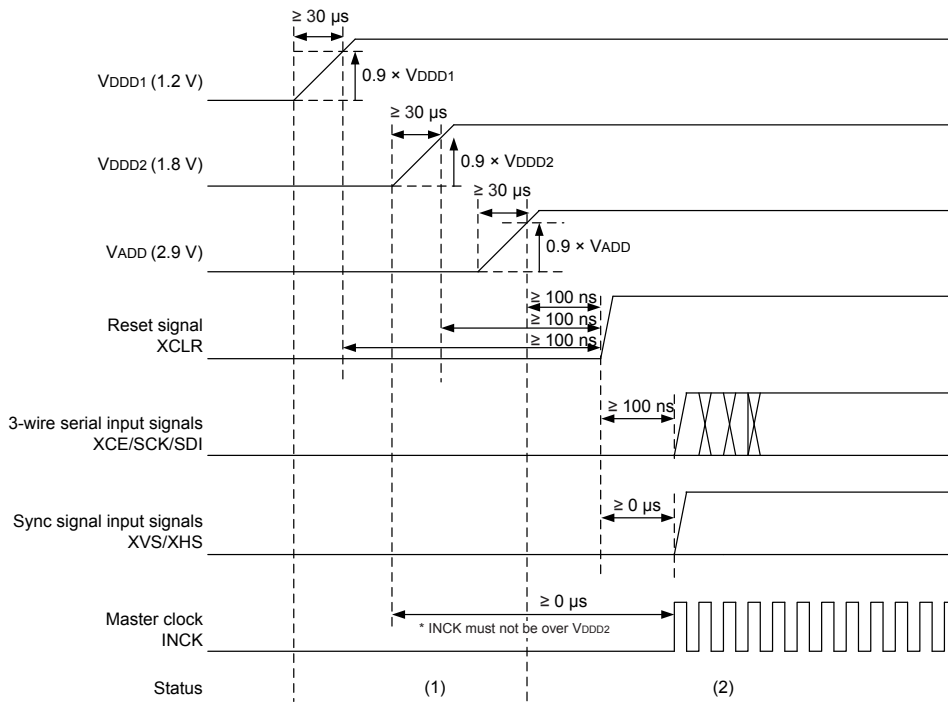
Power-on Sequence
