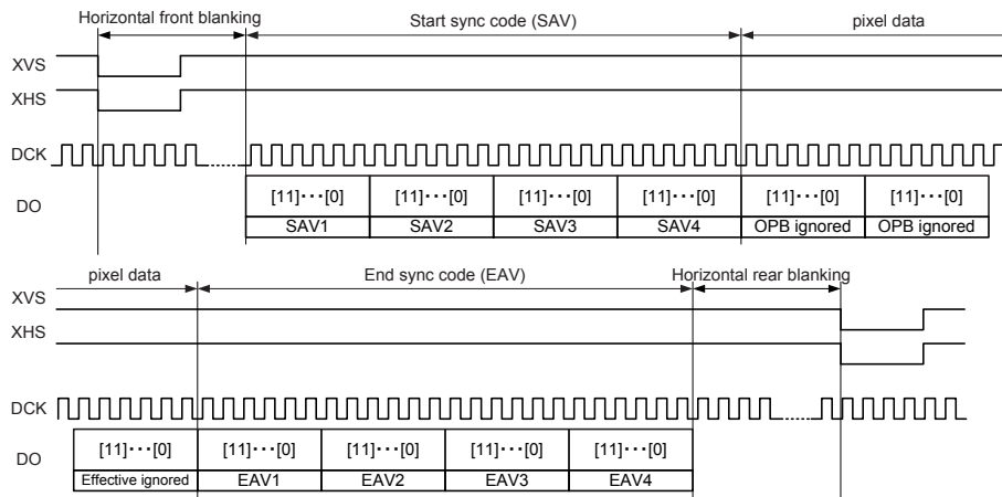
Sync Signal and Data Output Timing
