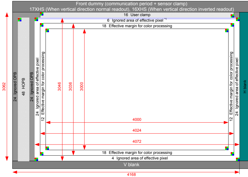
Readout Pixel Image Diagram (4000 × 3000)
