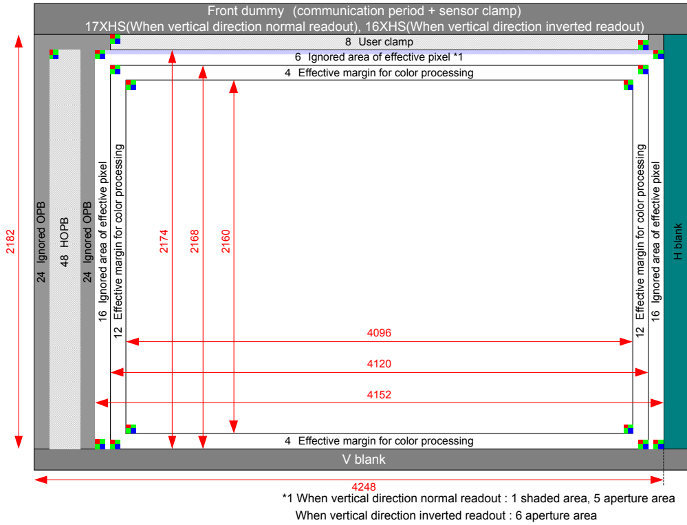
Readout Pixel Image Diagram (4096 × 2160)
