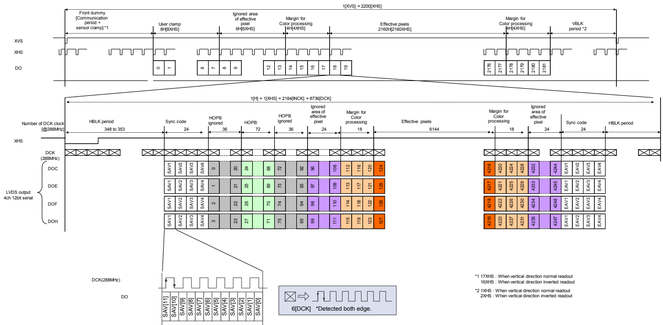
Readout Drive Timing
