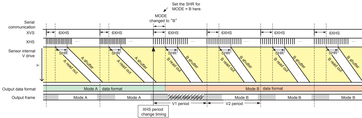
Mode Transition
