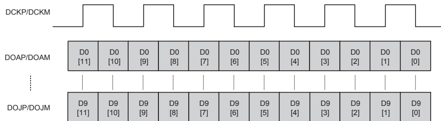
Serial Data Details (Sync Code Block)
